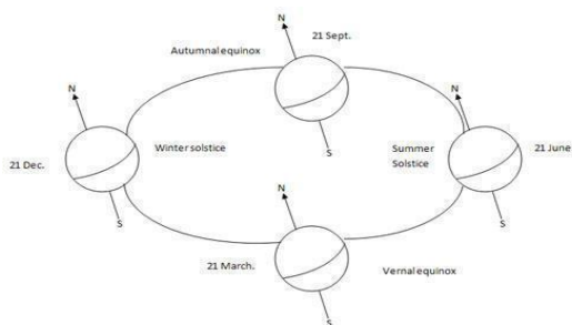
Fig. 1. The declination angles.
