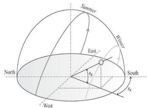
Fig. 2. Solar altitudes and azimuths typical behavior of sun path.
