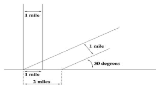
Fig. 3. One beam one mile wide shines on the ground at a 90^\circ angle, and another at a 30^\circ angle.
