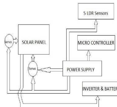
Fig. 4. Block diagram of overall system.
