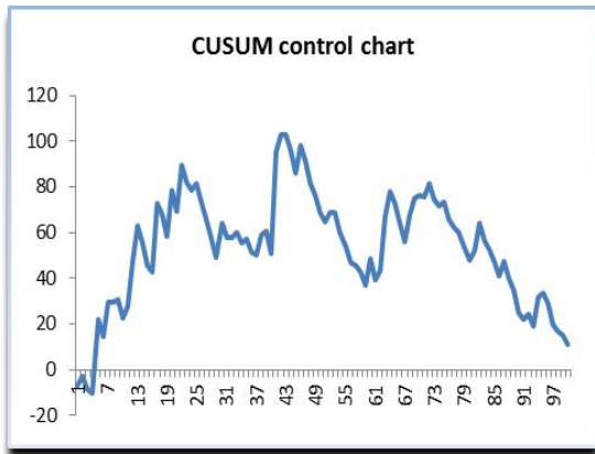
Fig. 6 The CUSUM control chart with reliability data
